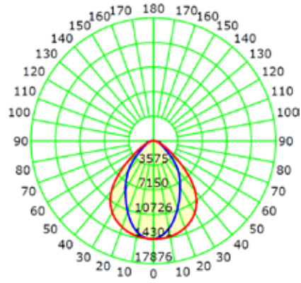
65°x95° (320W)
