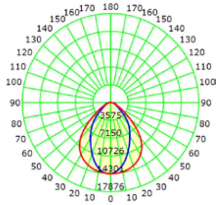
65°x95° (320W-HV)
