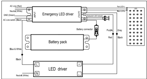
Wiring diagram (Maintained)
