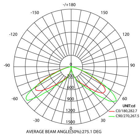
HL-BL-MW-MCCT-24W-DC (5000K)
