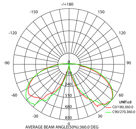
HL-BL-MW-MCCT-24W-CR (5000K)
