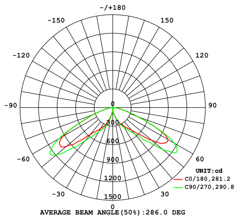
HL-BL-MW-MCCT-24W-DC (3000K)
