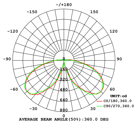
HL-BL-MW-MCCT-24W-CR (3000K)
