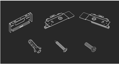
Wall Mounted Kit (HL-SLI-WM)
