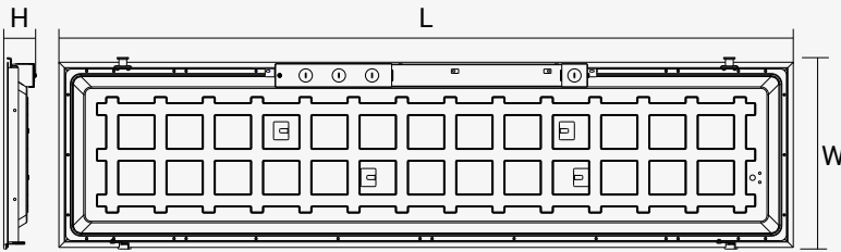
HL-2X2-MW-MCCT-40W-RETRO TROFFER
