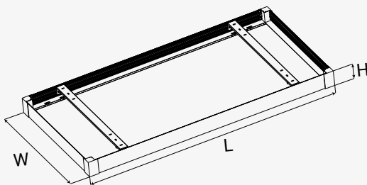
HL-RRP-RETRO PANEL-2X4 SURFACE KIT
